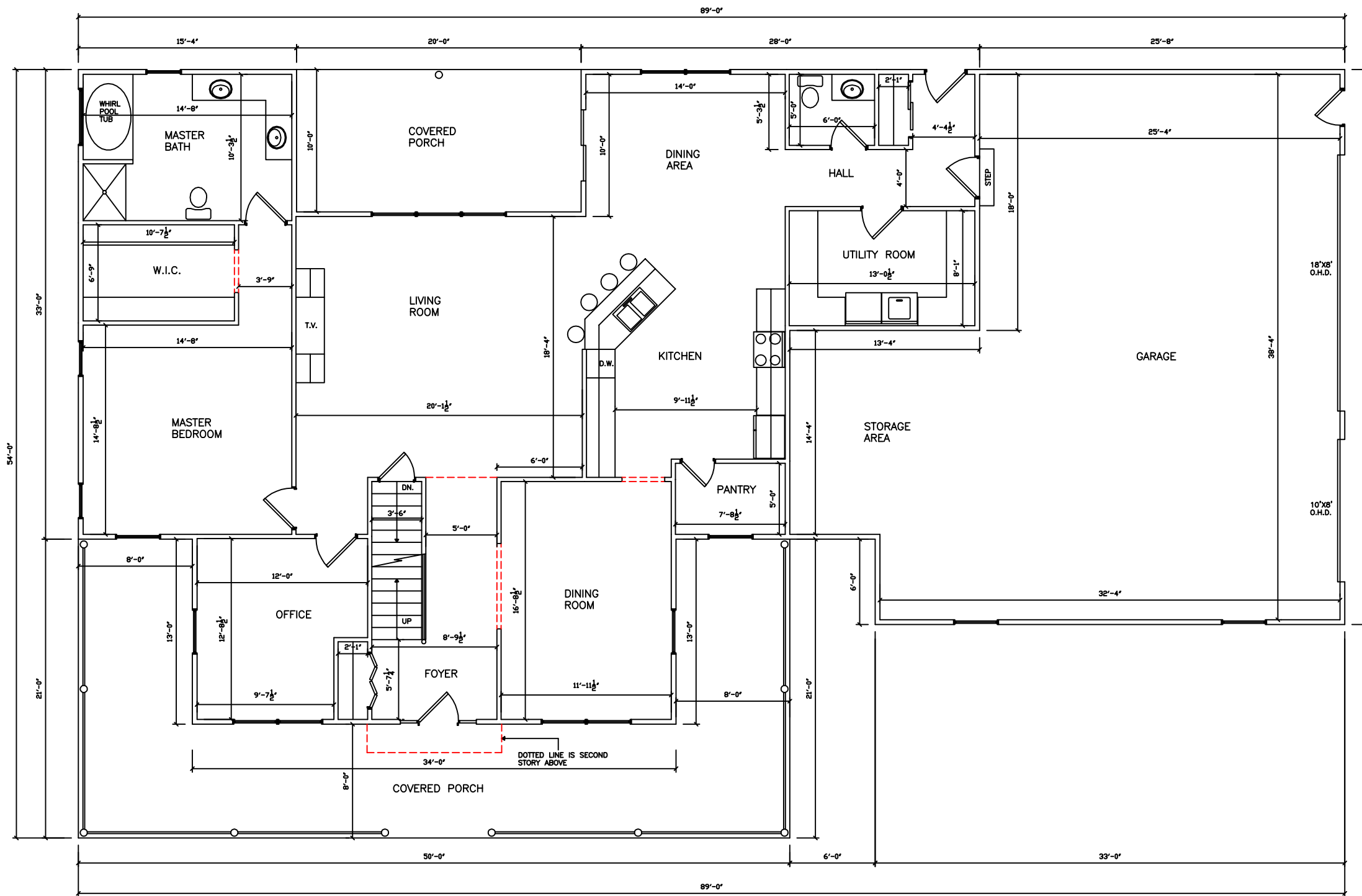
MAIN FLOOR PLAN SCALE 1/8" = 1'-0" 2137 SQ. FT.
